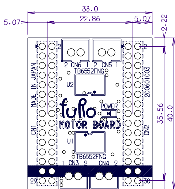
200601003 COMPONENT SIDE SILK
