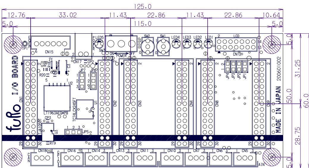
200601002 COMPONENT SIDE SILK 200601002 COMPONENT SIDE
